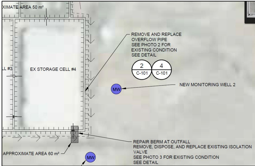
Cell 4 Work Plan
